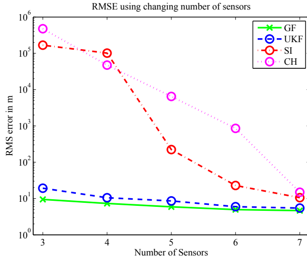
Figure 4: The RMSE with respect to the number of sensors used is shown. Logarithmic scale is used for the RMSE caused by the poor results of the least-squares approaches using too few sensors. The proposed Gaussian Estimator (green, solid) achieves best results, while the UKF (blue, dashed) is working almost as good as the GF. The SI (red, dot-dashed) shows poor results, as well as the CH (magenta, dotted).
